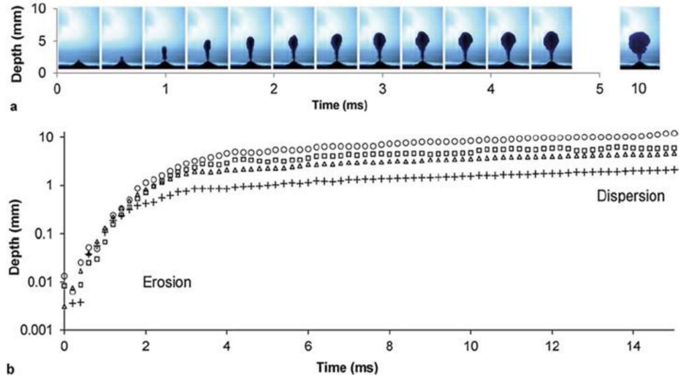
Fig. 4. Injection progress into acrylamide gel at constant jet speed. (a) Frames from a video recording of an injection ( 400\ \mu\text{s} apart, jet speed = 100\ \text{m/s} ); last frame shows dispersion at t = 10\ \text{ms} . (b) Injection progress at various constant jet speeds.
