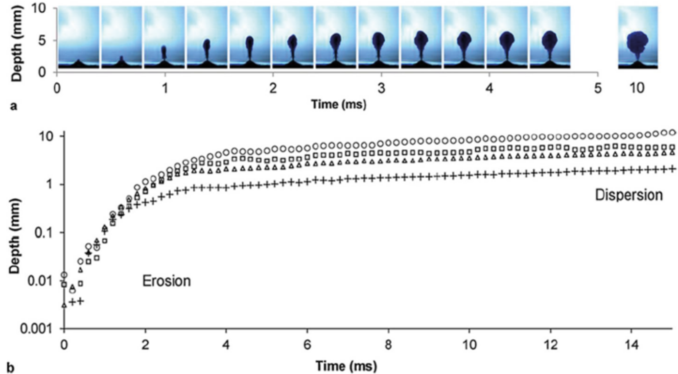
Fig. 4. Injection progress into acrylamide gel at constant jet speed. (a) Frames from a video recording of an injection ( 400 \mu\text{s} apart, jet speed = 100 \text{ m/s} ); last frame shows dispersion at t = 10 \text{ ms} . (b) Injection progress at various constant jet speeds.
